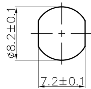
Panel cut
